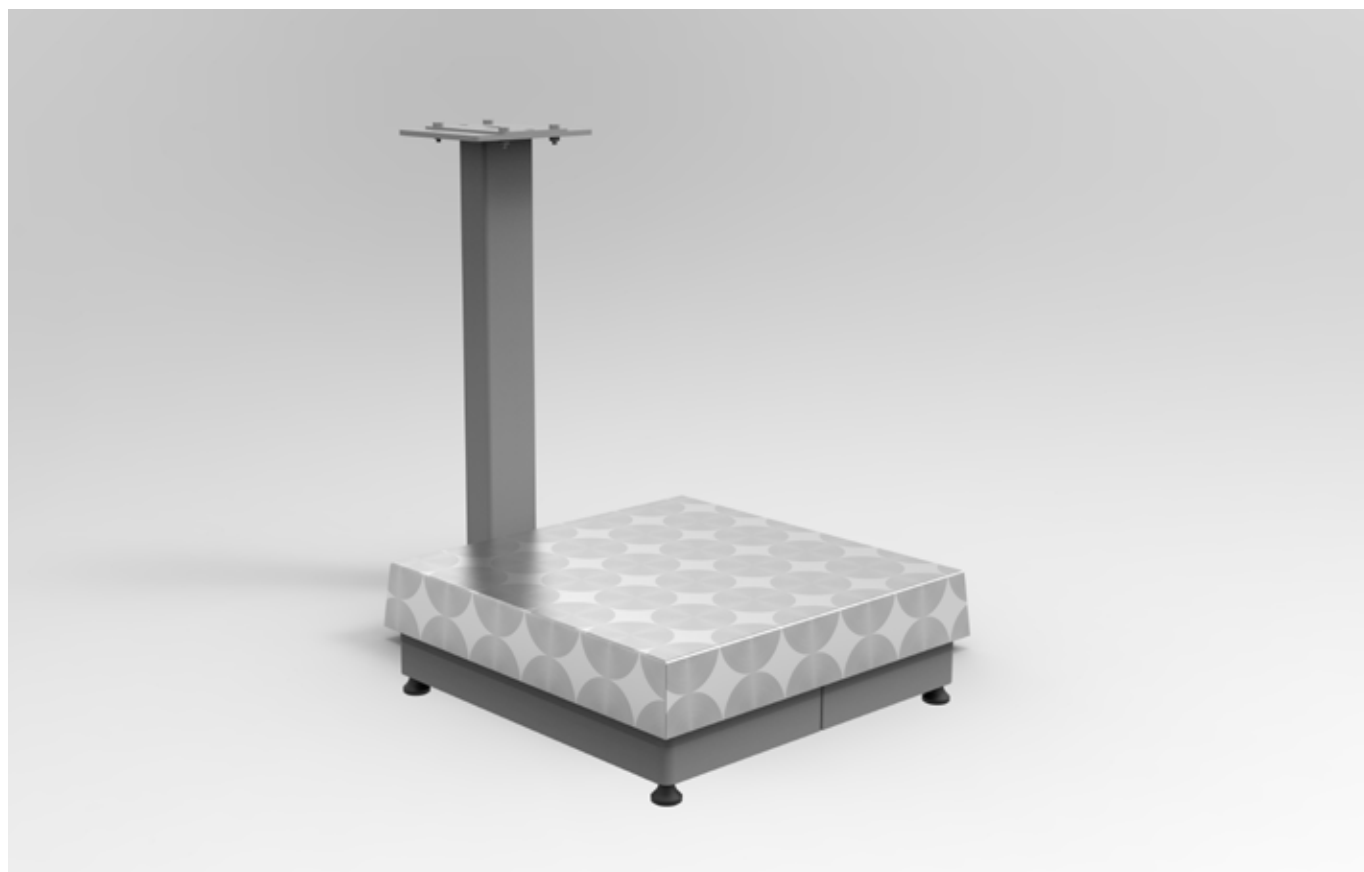
BT-BS-1818-100-SP Bench Scale Shown With (Optional) 24" Integral Column
