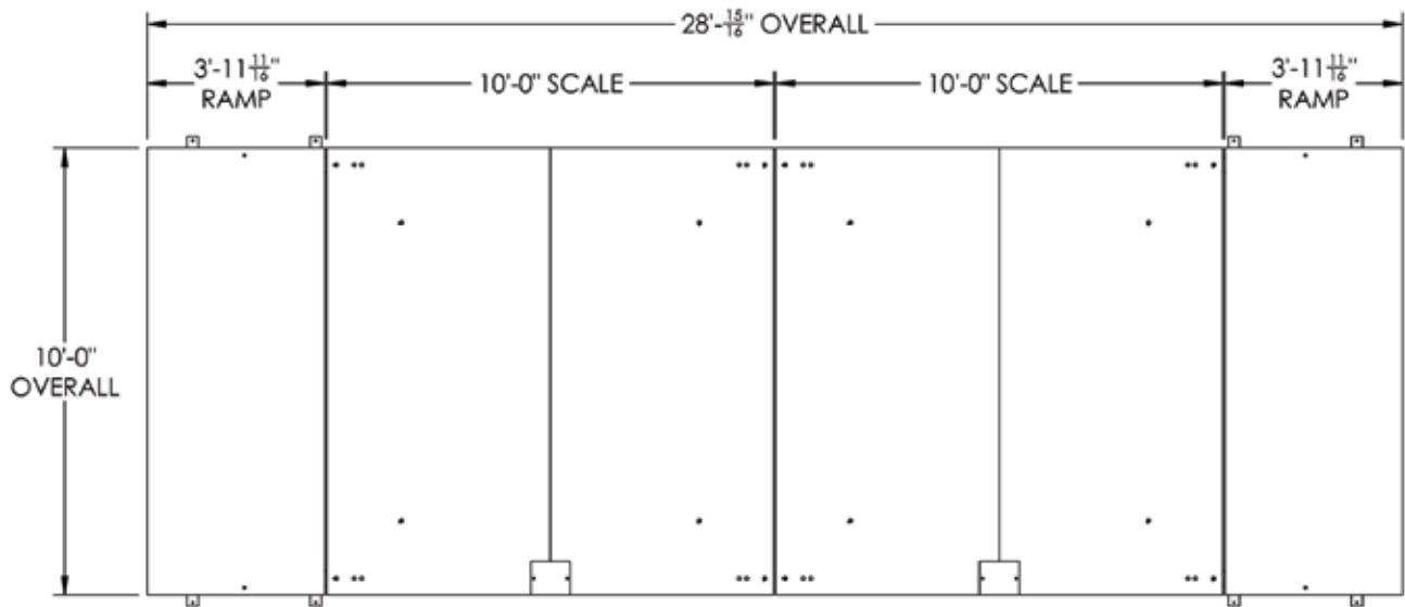
Drawing for 20' x 10' shown
